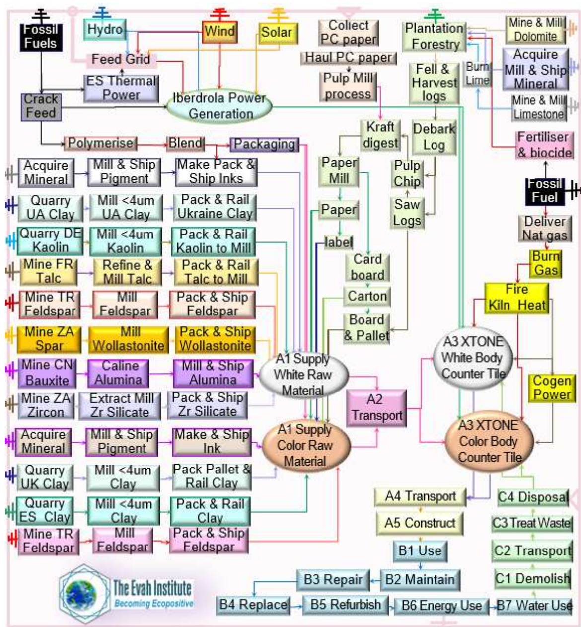
Figure 2 White & Colour Body Products Process Flow Charts
