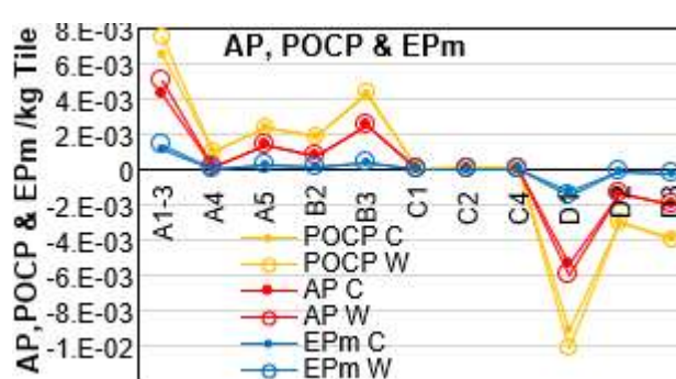
Figure 4 POCP Vs AP & EP/kg A to D3
