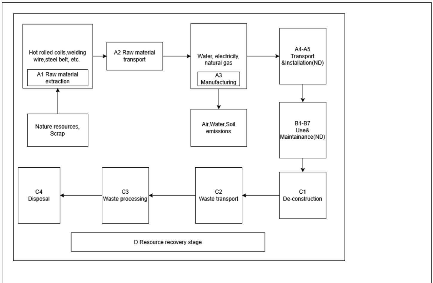
Figure 4: System Process Flow Chart
