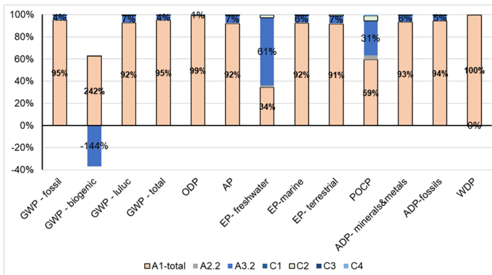
Figure 18: Life cycle impact contribution analysis- Structural built ups
