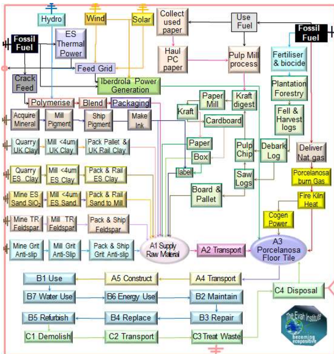
Figure 2. Product Process Flow Chart
